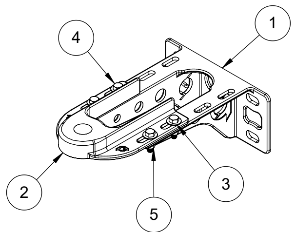
Mounting Detail
