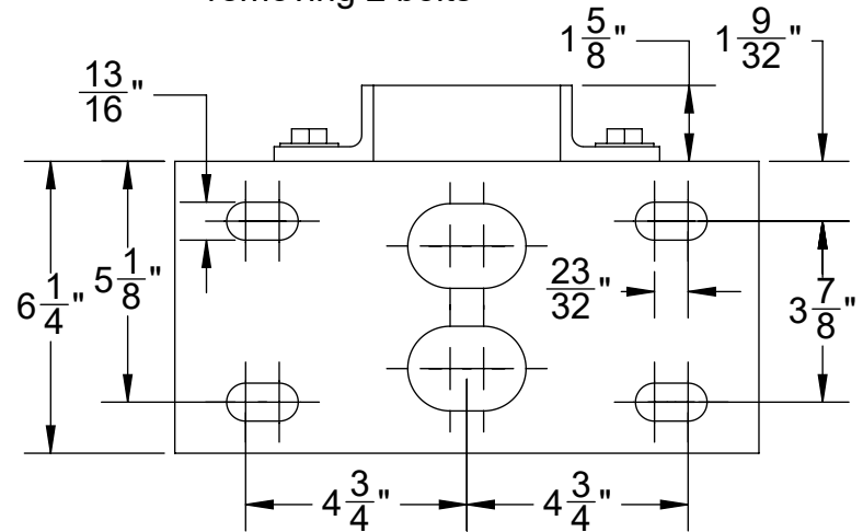
Mounting Detail
