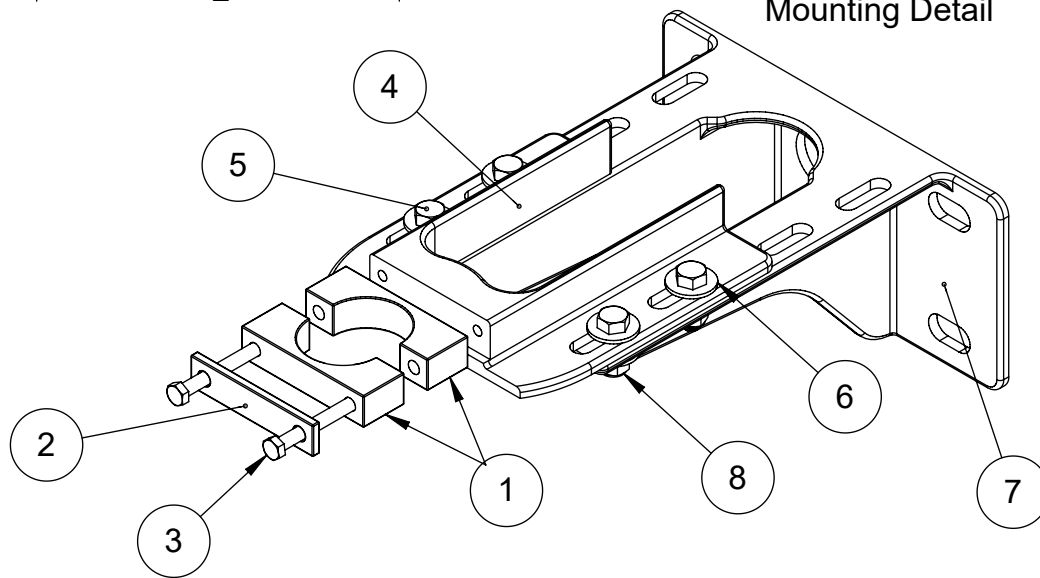
Mounting Detail
